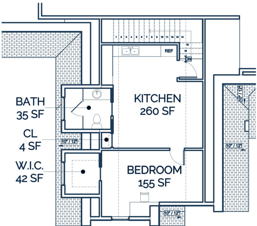
Bonus Room NTS
