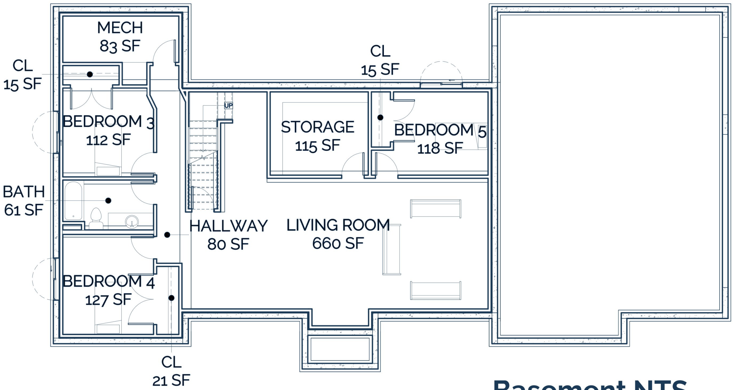
Basement NTS
