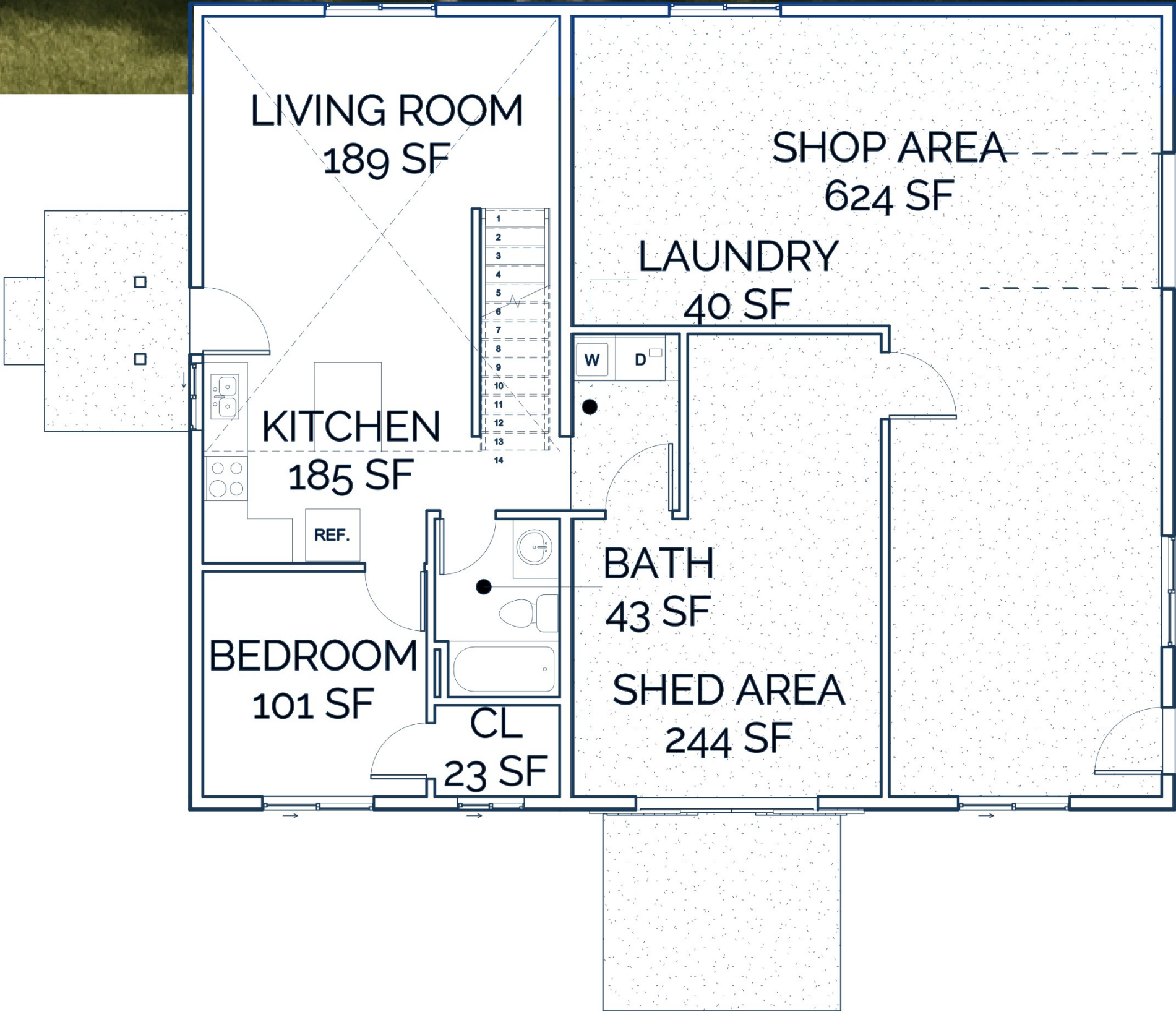
First floor NTS
